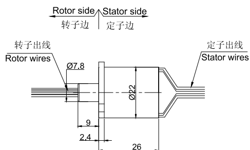
MC260-FL06图纸
