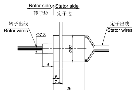
MC260-FL07图纸
